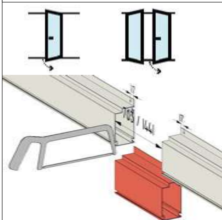
OPTION: HD (hinged door)
