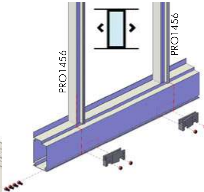
OPTION: SD (sliding door)
